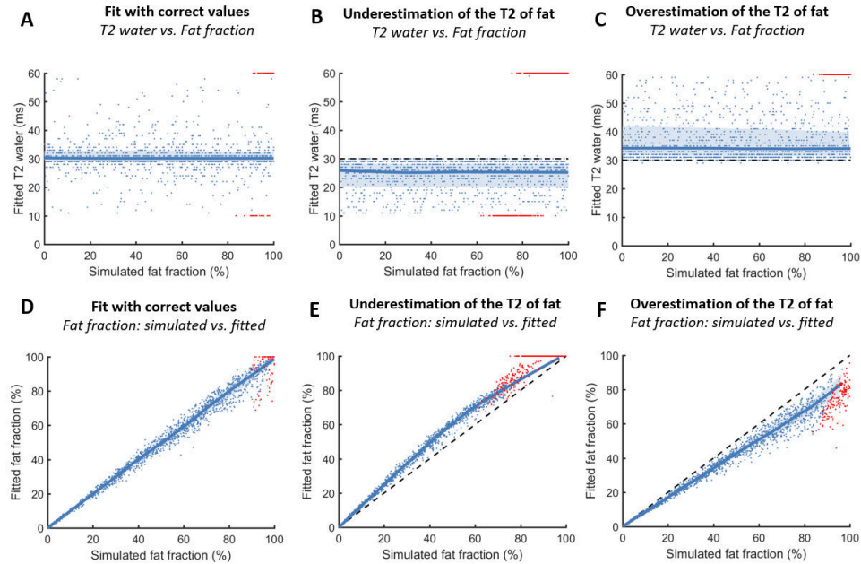
Figure 5. Simulation 2 shows the effect of fitting simulated data with different assumed T2_{\text{fat}} values. The top row shows the T2_{\text{water}} for assuming the correct T2_{\text{fat}} ( T2_{\text{water}} : median: 30 ms [23 ms – 38 ms], on dictionary boundaries: 4%, fig. A), an underestimation of T2_{\text{fat}} ( T2_{\text{water}} : median: 26 ms [14 ms – 30 ms], on dictionary boundaries: 26%, fig. B) and an overestimation of T2_{\text{fat}} ( T2_{\text{water}} : median: 33 ms [30 ms – 51 ms], on dictionary boundaries: 9%, fig. C). Fig. D, E and F show the relationship between the simulated FF and fitted FF. The values that fitted on dictionary boundaries are depicted in red and the correctly fitted values are depicted in blue. A reference line is shown at a T2_{\text{water}} of 30 ms and a unity line is shown for the fat fractions.
